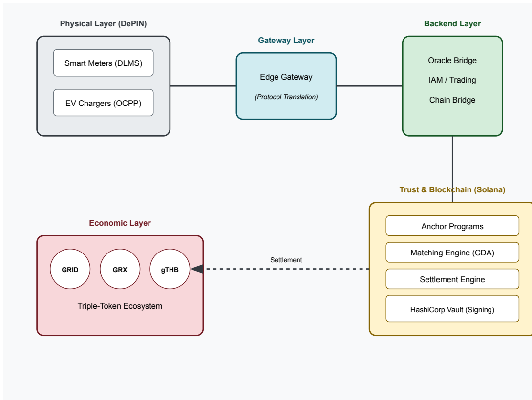
Figure 1: The GridTokenX multi-layer architecture spanning DePIN hardware to Solana settlement.
